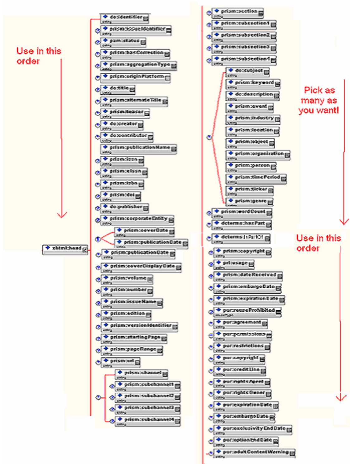
Figure 2 Structure of the elements in the article head
