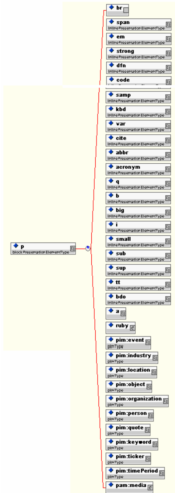
Figure 4. Block Presentation Element Structure
