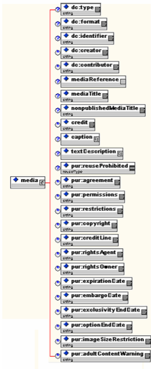
Figure 5 PAM Media Element
