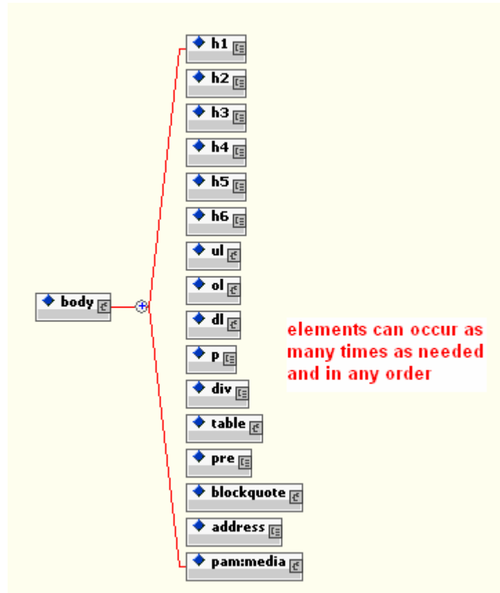
Figure 3 PAM Body Elements
