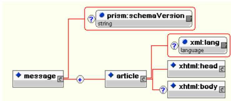
Figure 1 PAM Message Framework
